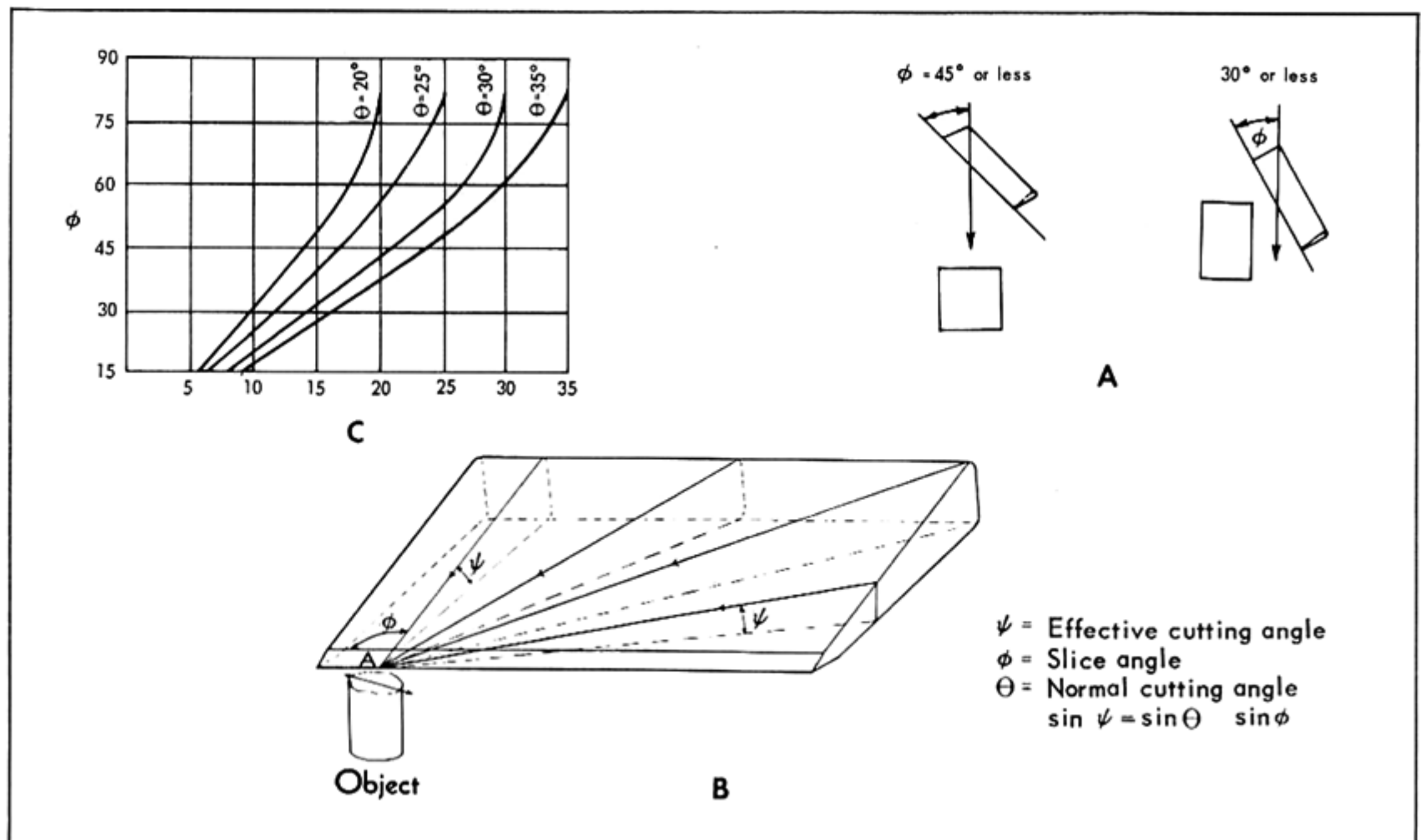
Fig. 15. A. Showing slice angle ( \phi ) for square and rectangular blocks. B. Decreased wedging with small slice angles. C. The relations between them plotted with permission from data of Preston (1933).
