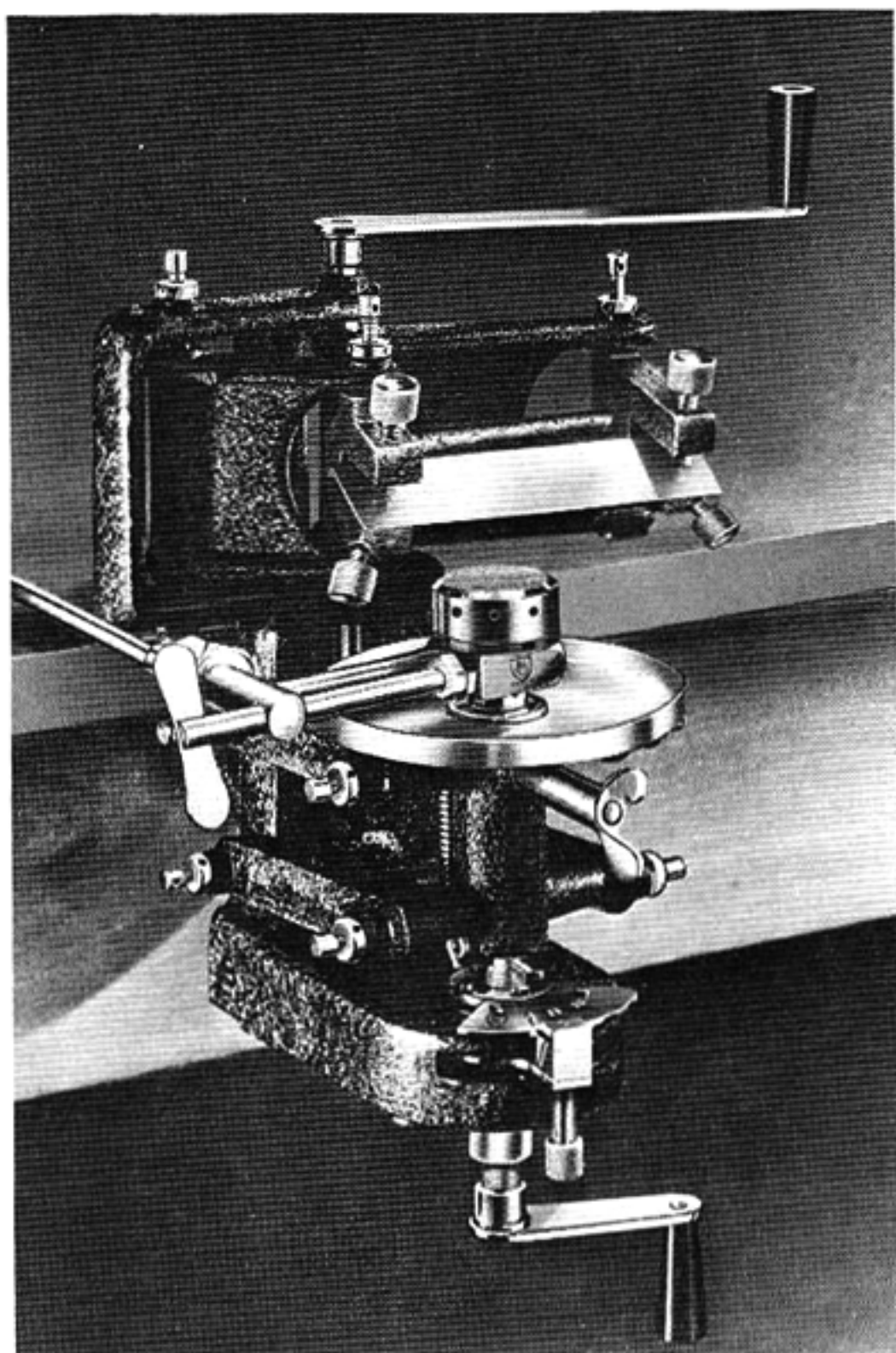
Fig. 18. AO 888 Automatic Clinical Microtomes and 930 Freezing Attachment.
