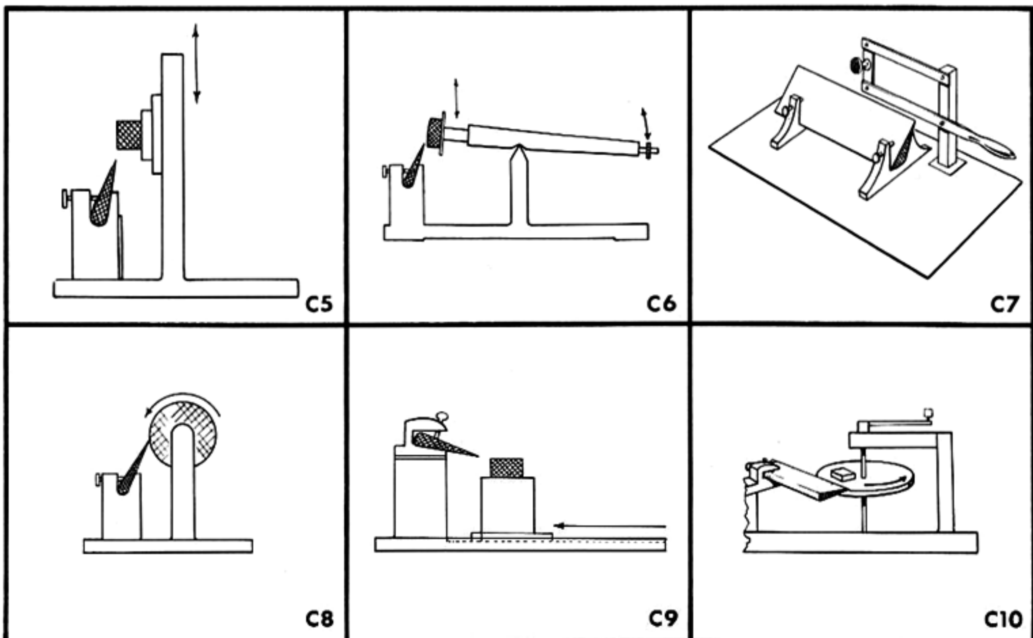
Types of microtome mechanisms.
