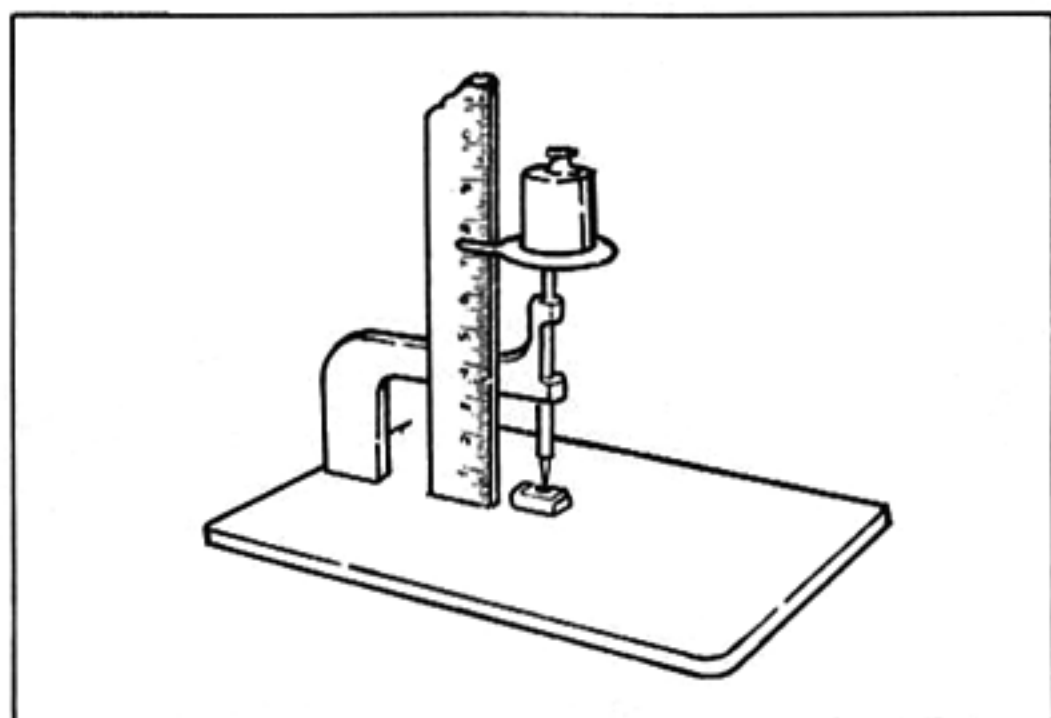
Fig. 21. Penetrometer for measuring hardness of specimens.
