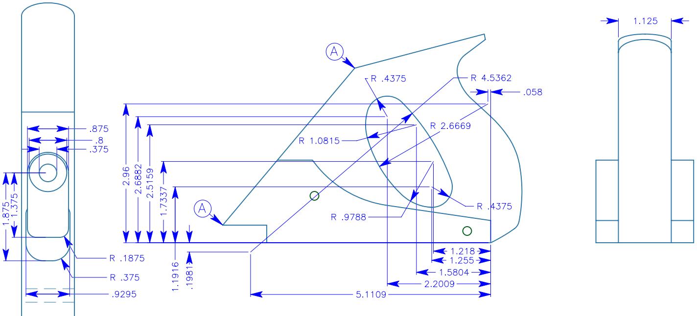
Adjuster Mortise View from A-A
