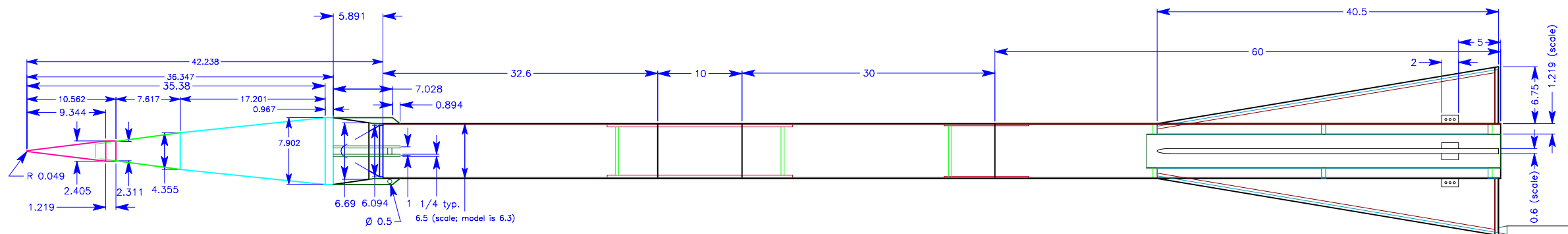
ASP 2 Supersonic Diffuser nose cone
